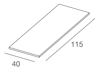
WSME mensola in nobilitato chipboard shelf L115 x P40 cm – sp 18 mm
