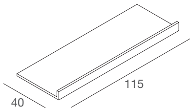
WSMEI mensola inclinata in nobilitato sloping chipboard shelf L115 x P40 cm – sp 18 mm
