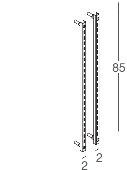
WGCRE coppia cremagliere per pannello Wall Gallery pair of racks for Wall Gallery
