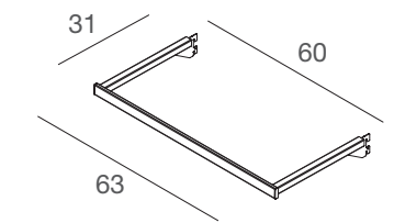
WSBAP3 barra appenderia in metallo metal hanging bar L.63 cm x P. 31 cm
