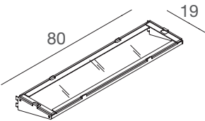
WGME6 mensola in vetro compresa di reggimensola in ferro glass shelf with iron shelf holders
