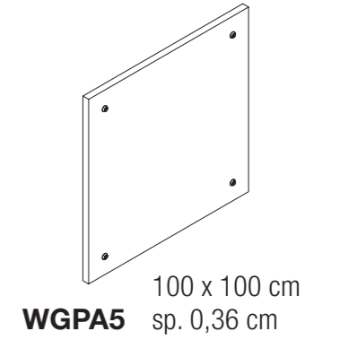
PANNELLO IN NOBILITATO SP.36 mm CON 4 BOCCOLE CHIPBOARD PANEL TH.36 mm WITH 4 PLUGS
