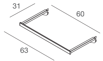
WSBAP3 barra appenderia in metallo metal hanging bar L.63 cm x P. 31 cm
