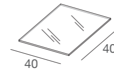
WSMEM/V mensola media in vetro temperato medium tempered glass shelf L40 x P40 cm – sp 8 mm
