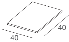
WSMEM mensola media in nobilitato chipboard shelf L40 x P40 cm – sp 18 mm
