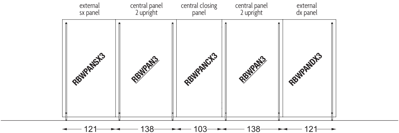
SCHEMA MONTANTI PASSO 120 DIAGRAM UPRIGHTS PITCH 120
