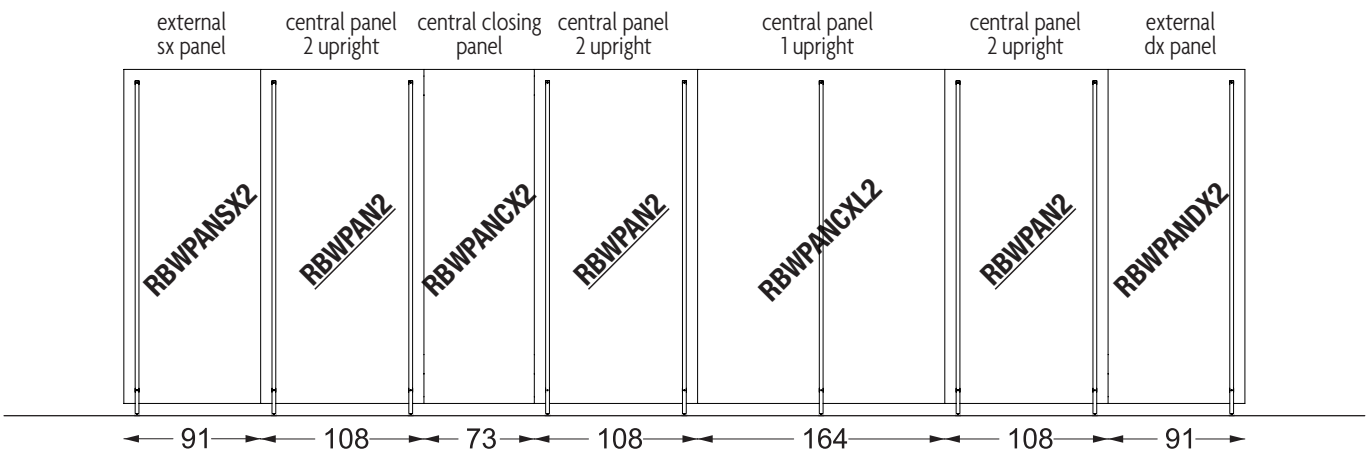
SCHEMA MONTANTI PASSO 90 DIAGRAM UPRIGHTS PITCH 90
