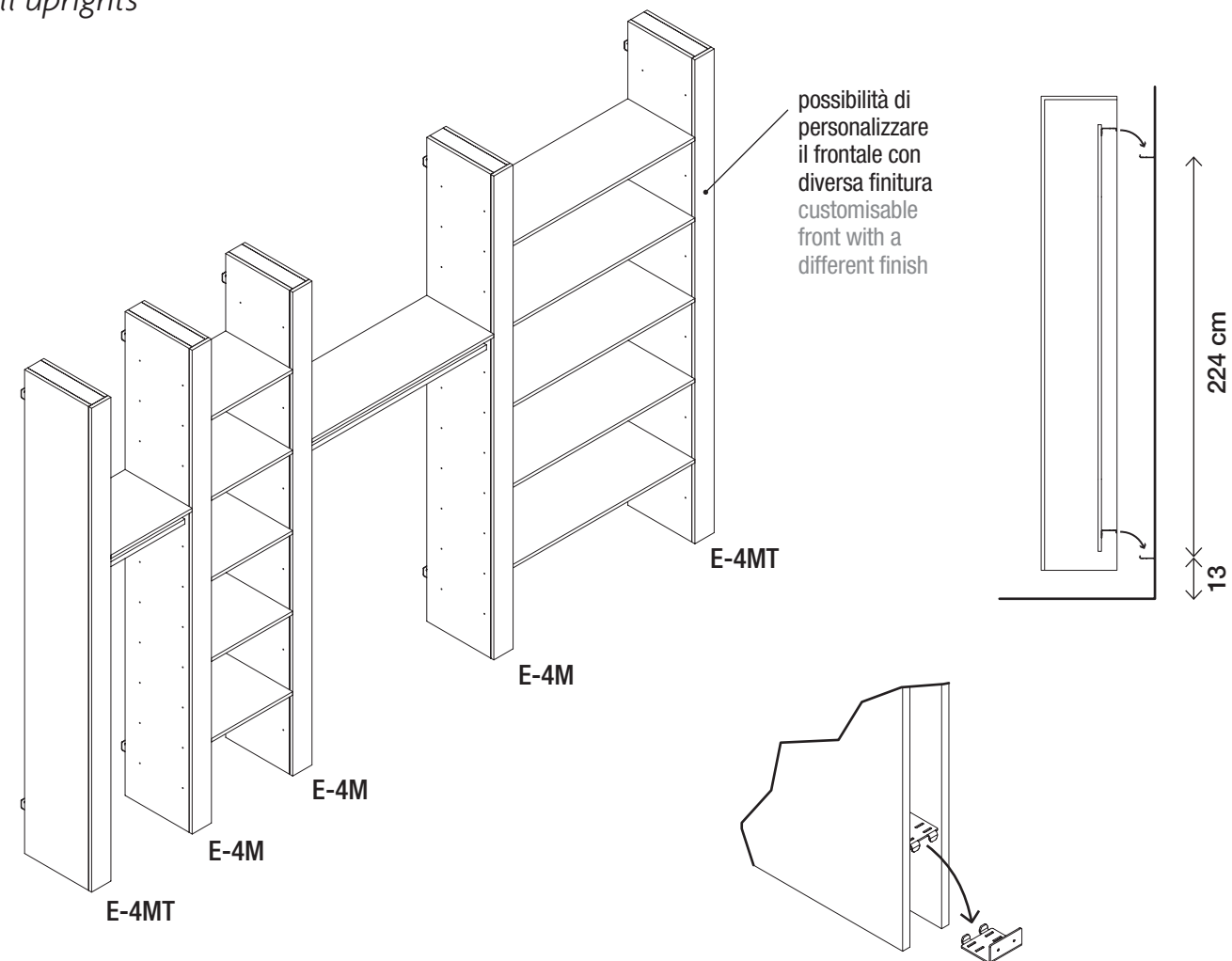
staffa fissata a parete wall fixing bracket
