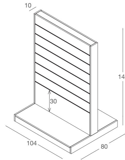
DGGD gondola dogata in nobilitato chipboard middle unit L104 x P80 x H145 cm
