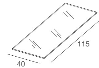
DGME/V mensola in vetro temperato tempered glass shelf L115 x P40 x SP0,8 cm
