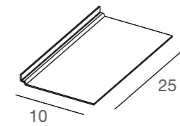
DGMA25 mensola in PMMA trasparente PMMA transparent acrylic shelf L25 x P10 cm
